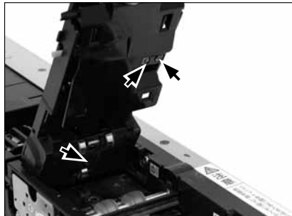
搬送路下側
